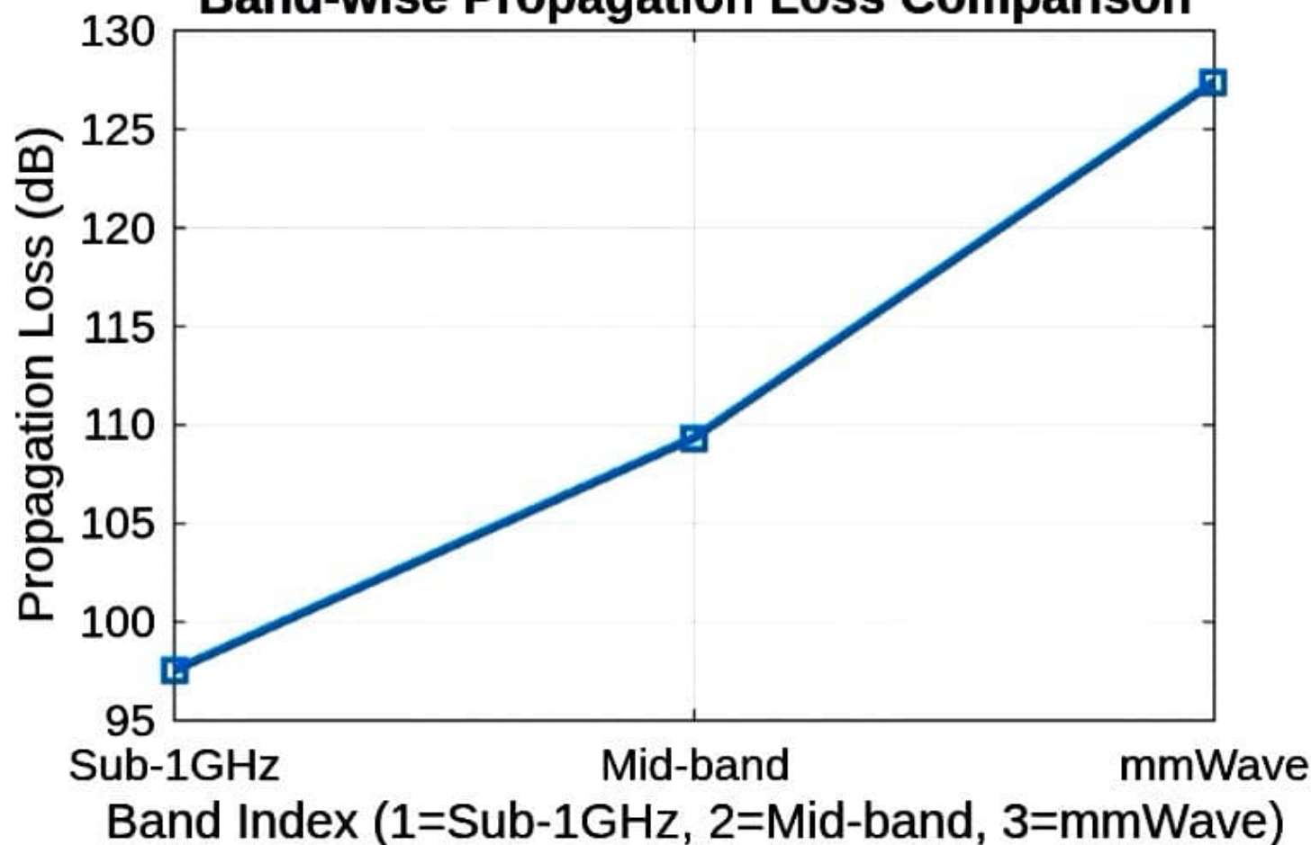
Band-wise Propagation Loss Comparison
