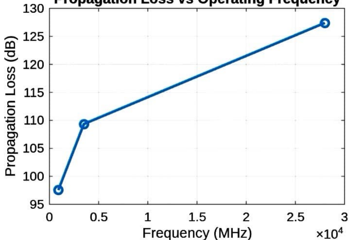
Propagation Loss vs Operating Frequency
