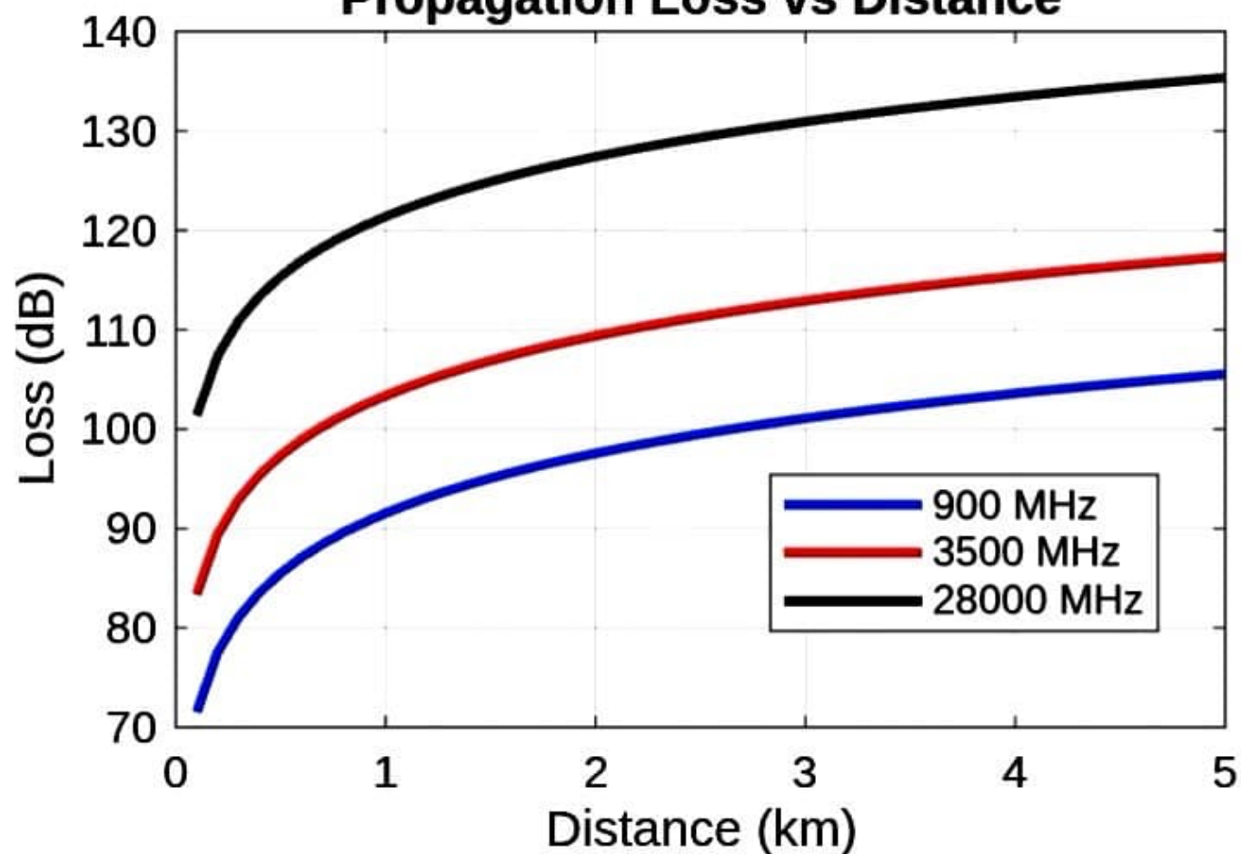
Propagation Loss vs Distance
